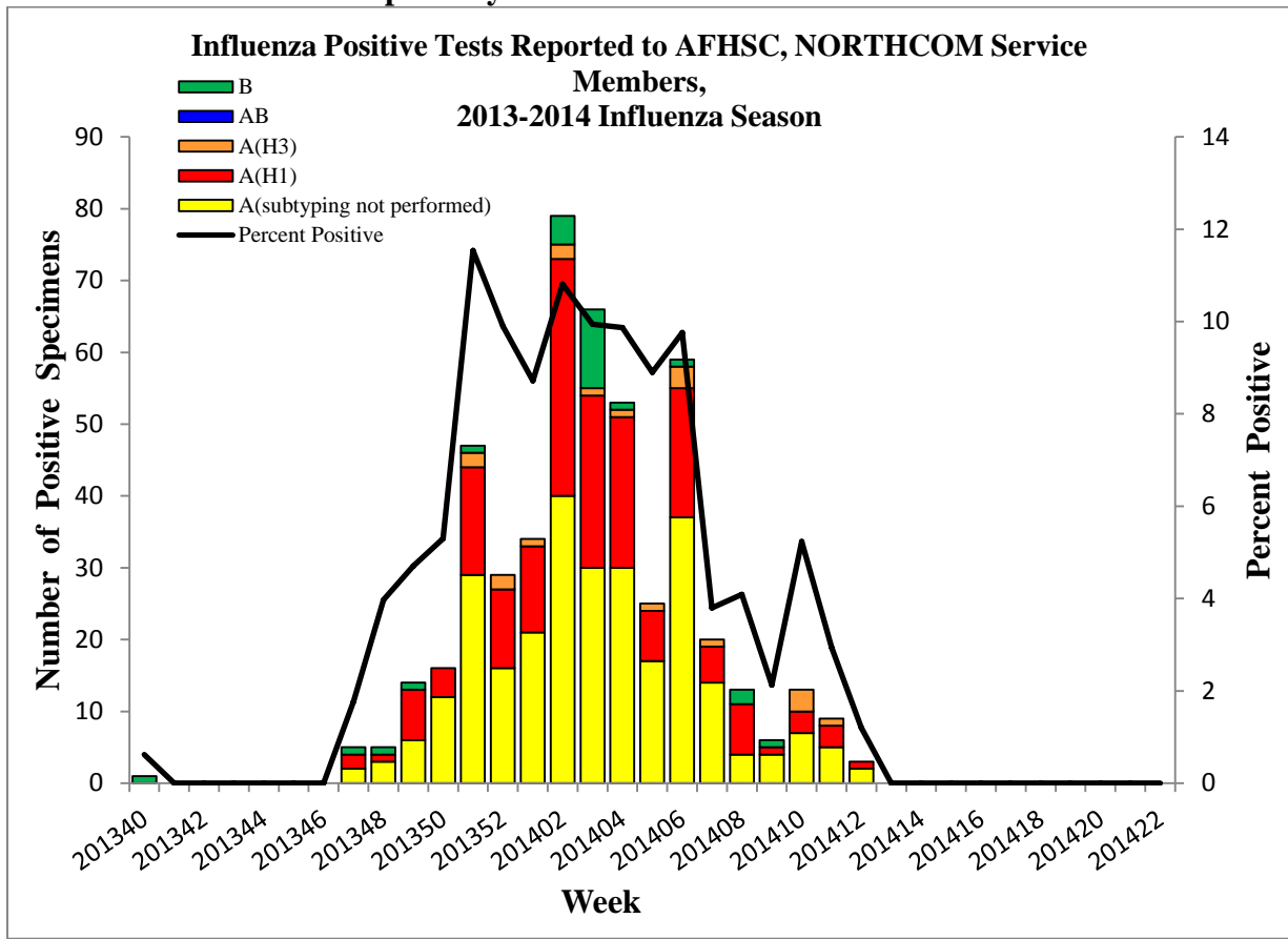
Figure 1d. Influenza Positive Tests Reported in Health Level 7 data: Service Members and Other Beneficiaries Presented Separately
